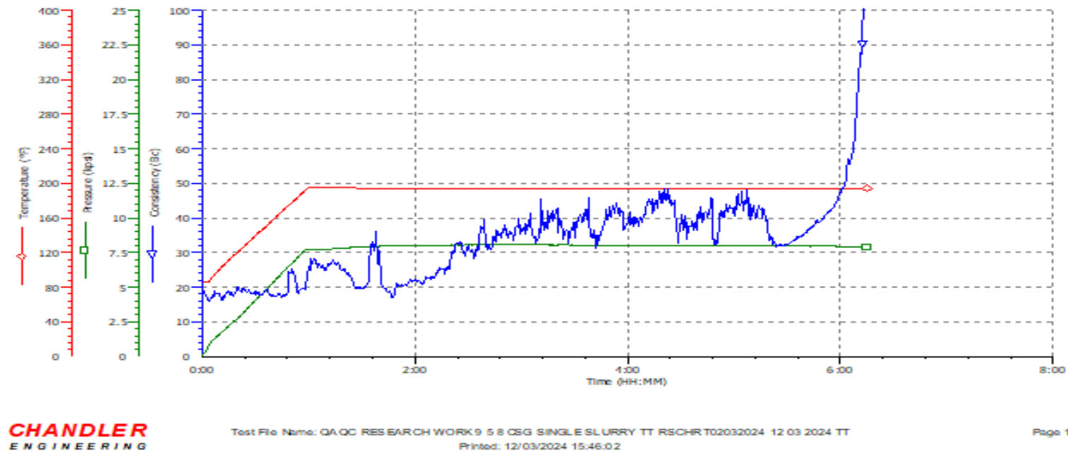
Fig. 7. Thickening Time for 0.5% bwoc of locally synthesized retarder
