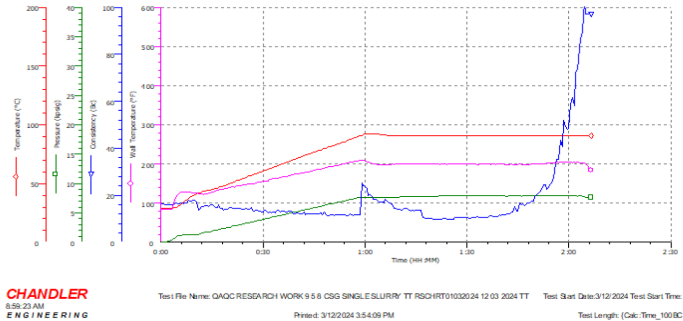
Fig. 5. Thickening Time for Neat Slurry
