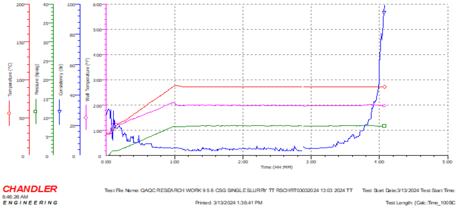
Fig. 6. Thickening Time for 0.3% bwoc of locally synthesized retarder
